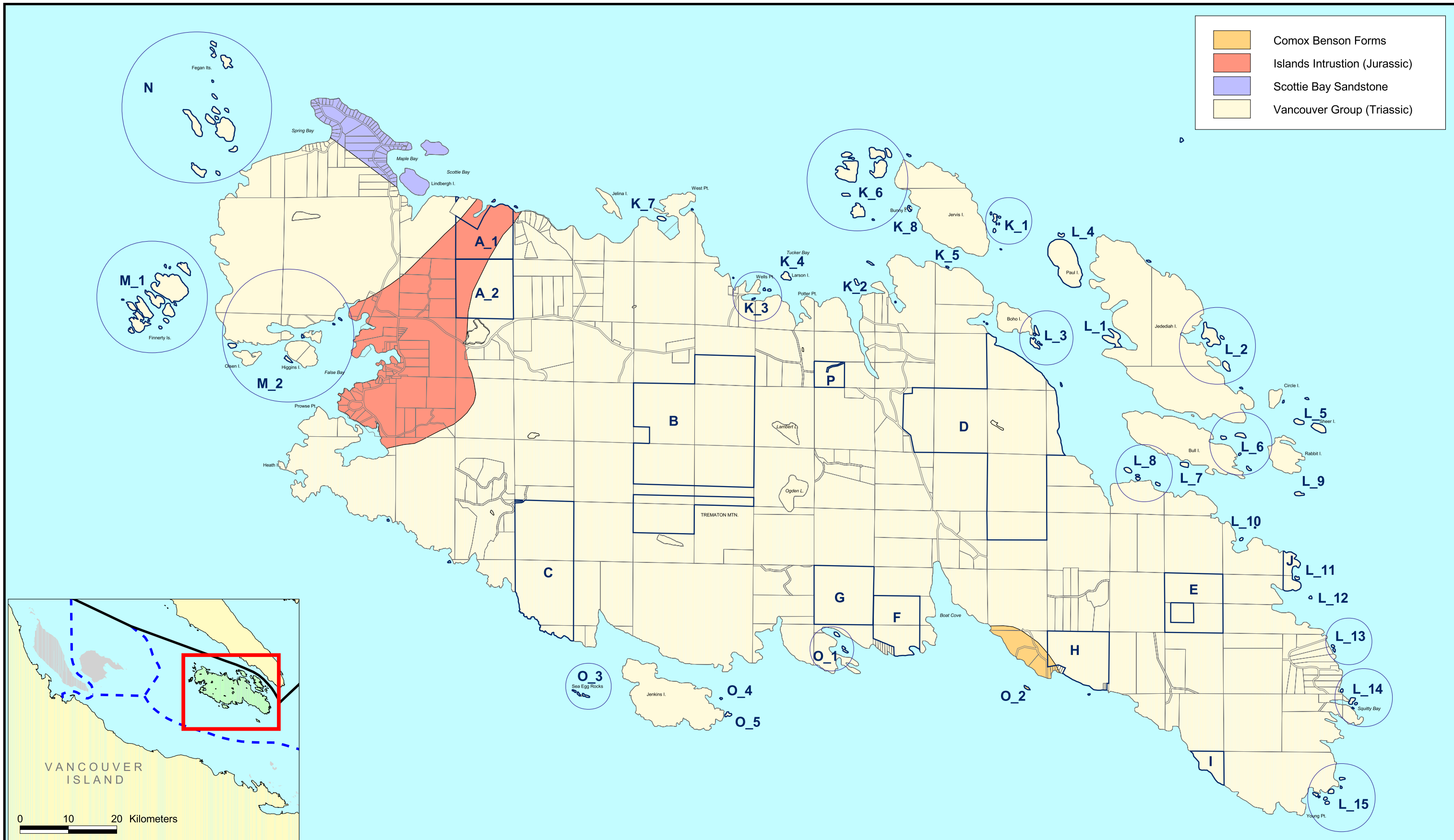
Map 3. Geology Parcels A through P and associated Sub Areas Geology data based on small scale map provided by Ministry of Energy and Mines. 2 0 2 4 Kilometers Scale 1:50,000 N
