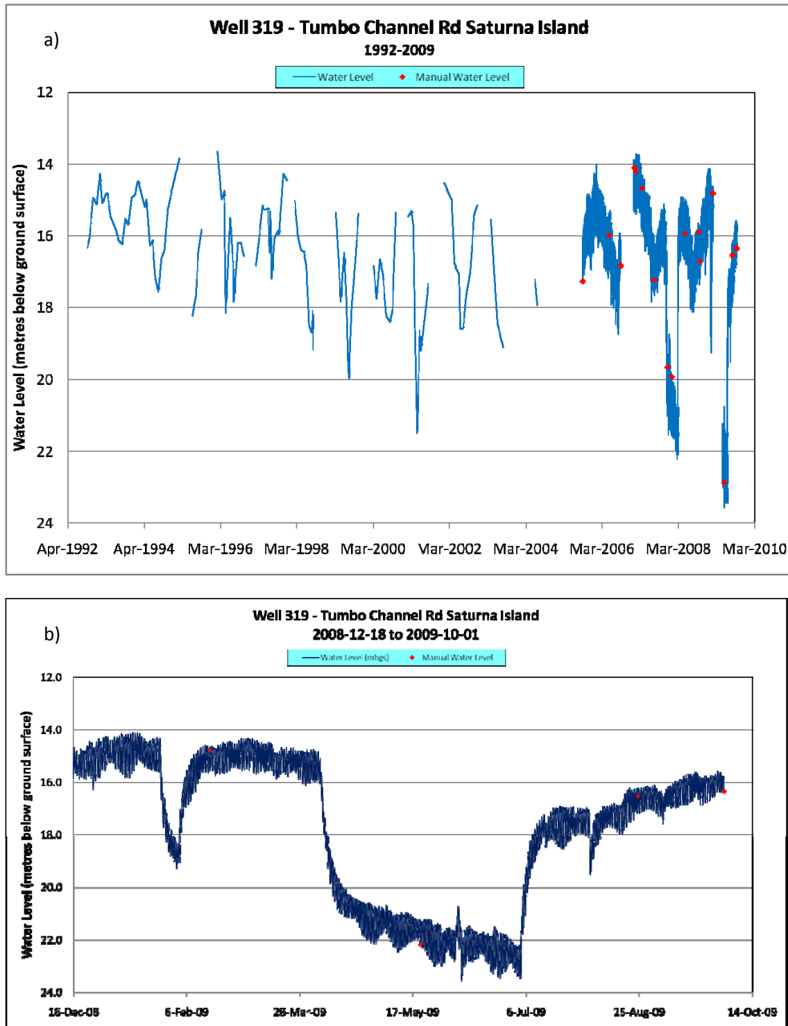
Figure 6. Hydrographs for Observation Well 319: (a) complete record of water level measurements in the monitoring well between May 1992 and August 2009 and (b) water level variation between December 2008 and October 2009, highlighting the water level decline between April and July 2009.
