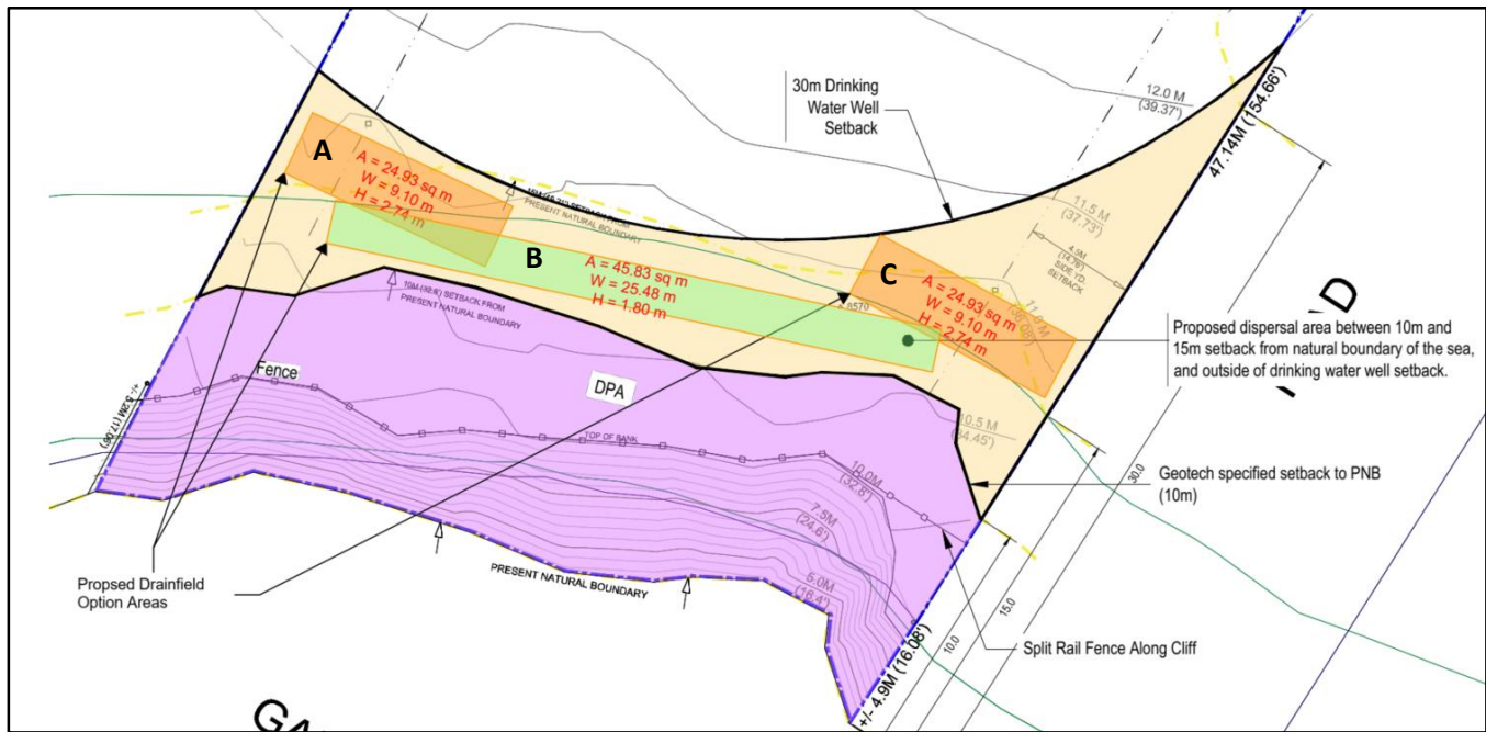
Figure 3 – Septic Field Options (A, B, and C)
